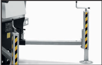
4 adjustable stabilizers.
