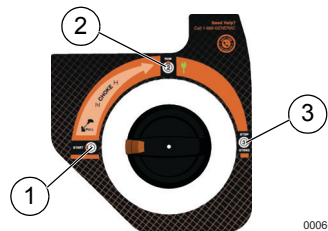
Figure 3-2. PowerDial Positions
